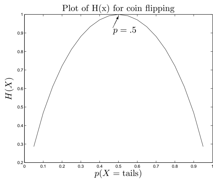
Figure 2: Entropy is maximal for the uniform distribution
